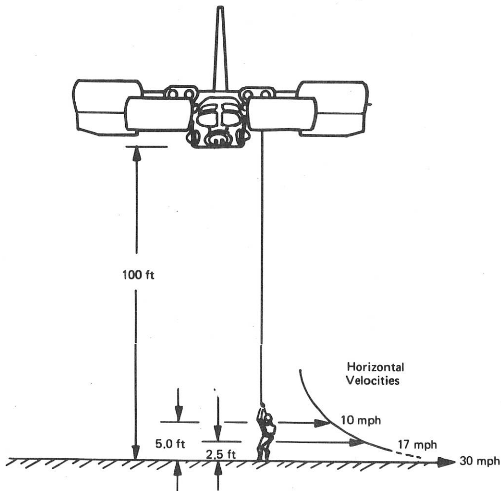
Downwash Characteristics of the X-22A Aircraft
