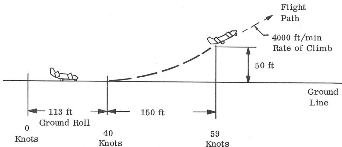
Profile of a Typical Maximum Performance Short Take-Off
