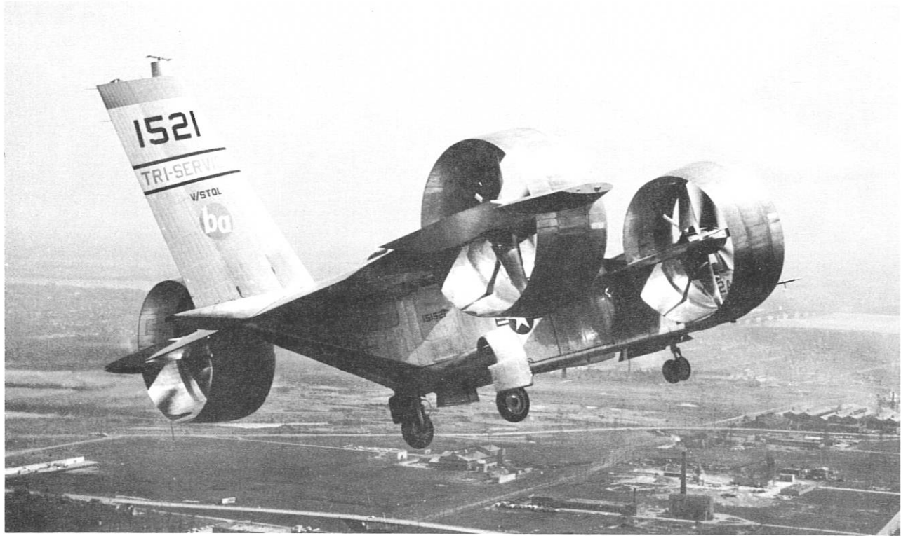
X-22A TRI-SERVICE DUAL TANDEM DUCTED PROPELLER V/STOL RESEARCH AIRCRAFT
