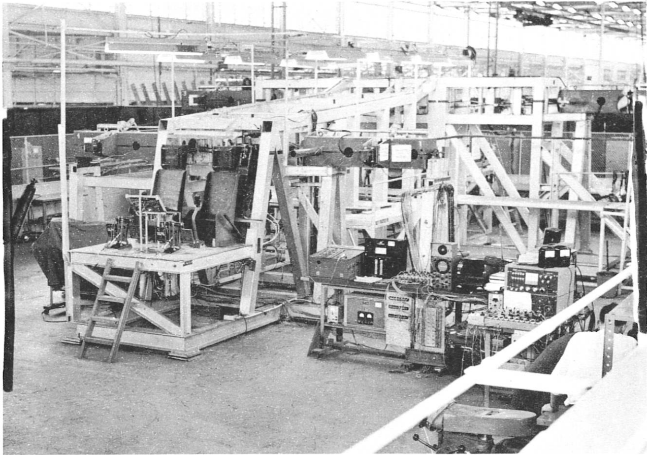
Control System Test Stand
