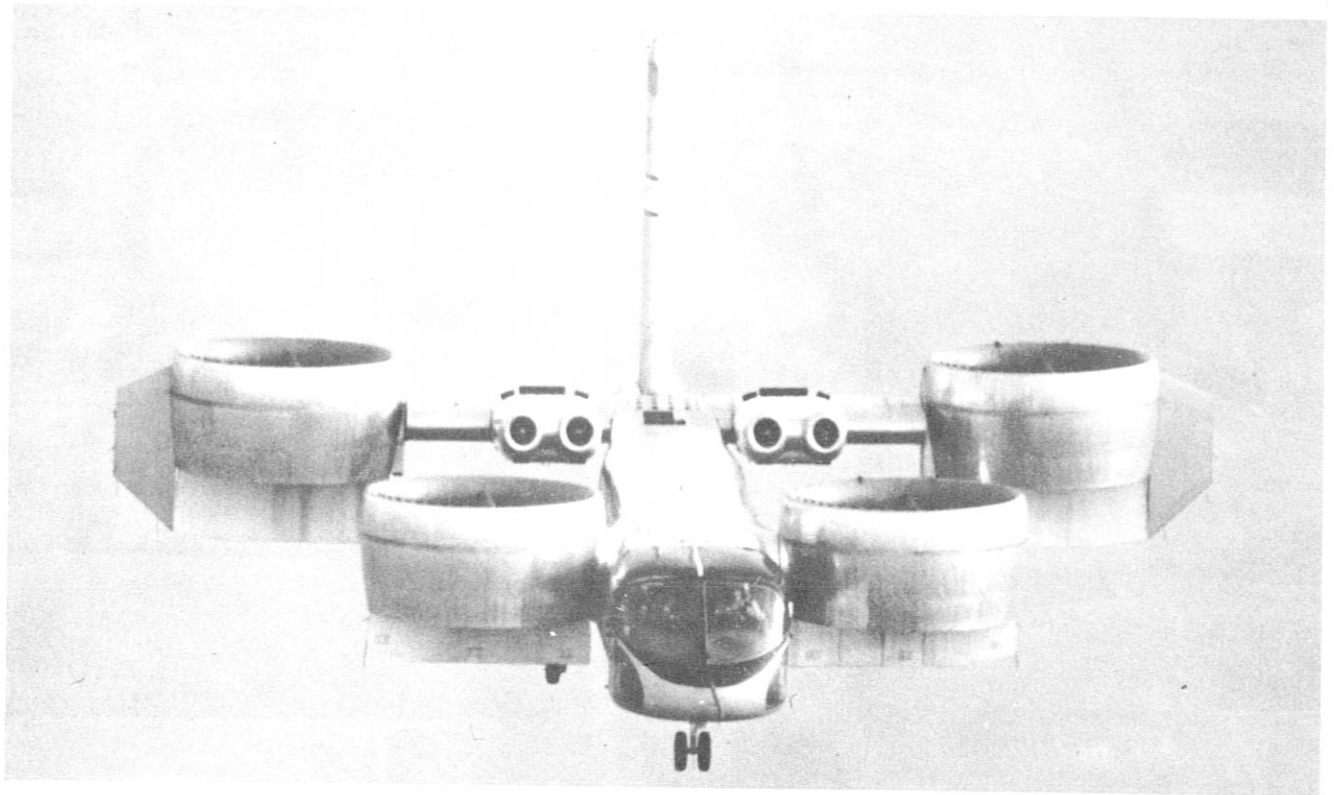
Hovering at Altitude - Front View
