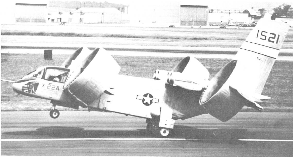
STOL - Short Landing - 30° Duct Angle
